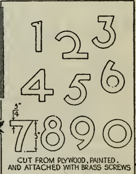
SCROLL-SAWED FROM 1/4" PLYWOOD
