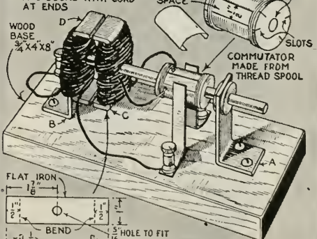
② SERIES MOTOR
